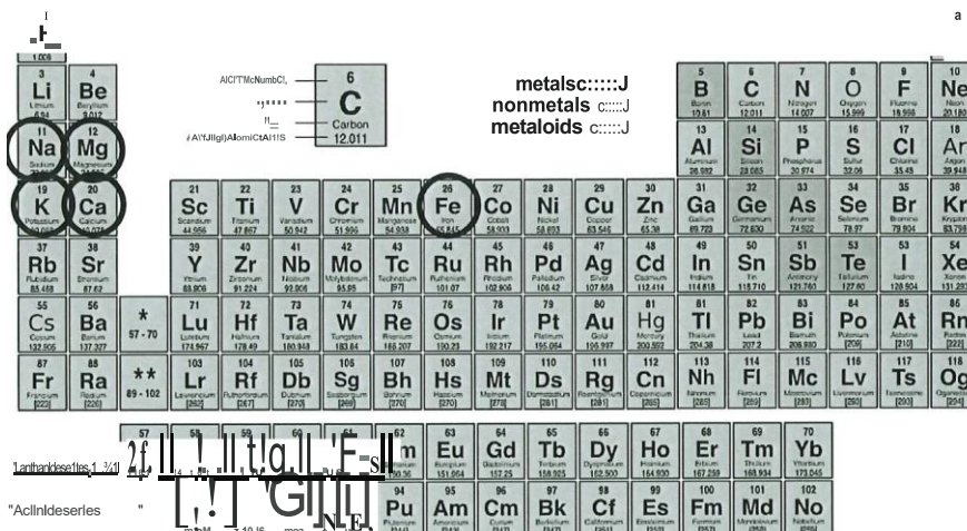
The location of some metals in the periodic table which have important ions in the body
